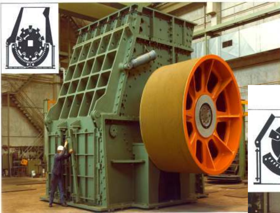
MAMMUT SINGLE-SHAFT HAMMER CRUSHER
