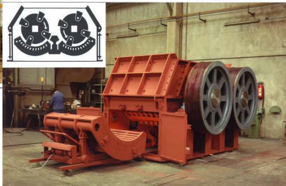
TITAN DOUBLE-SHAFT HAMMER CRUSHER
