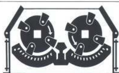
TITAN DOUBLE-SHAFT HAMMER CRUSHER
